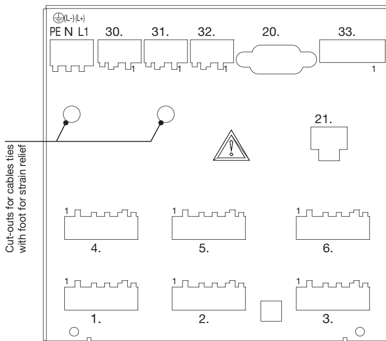
Rear view of a 3/6-channel paperless recorder with pluggable screw terminals
